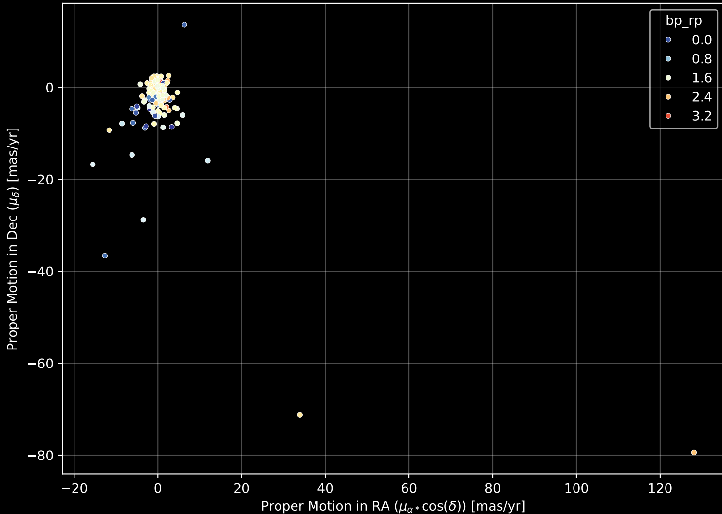
APOGEE DR17 Field: [206-04] Proper Motion Diagram (n= 208)
