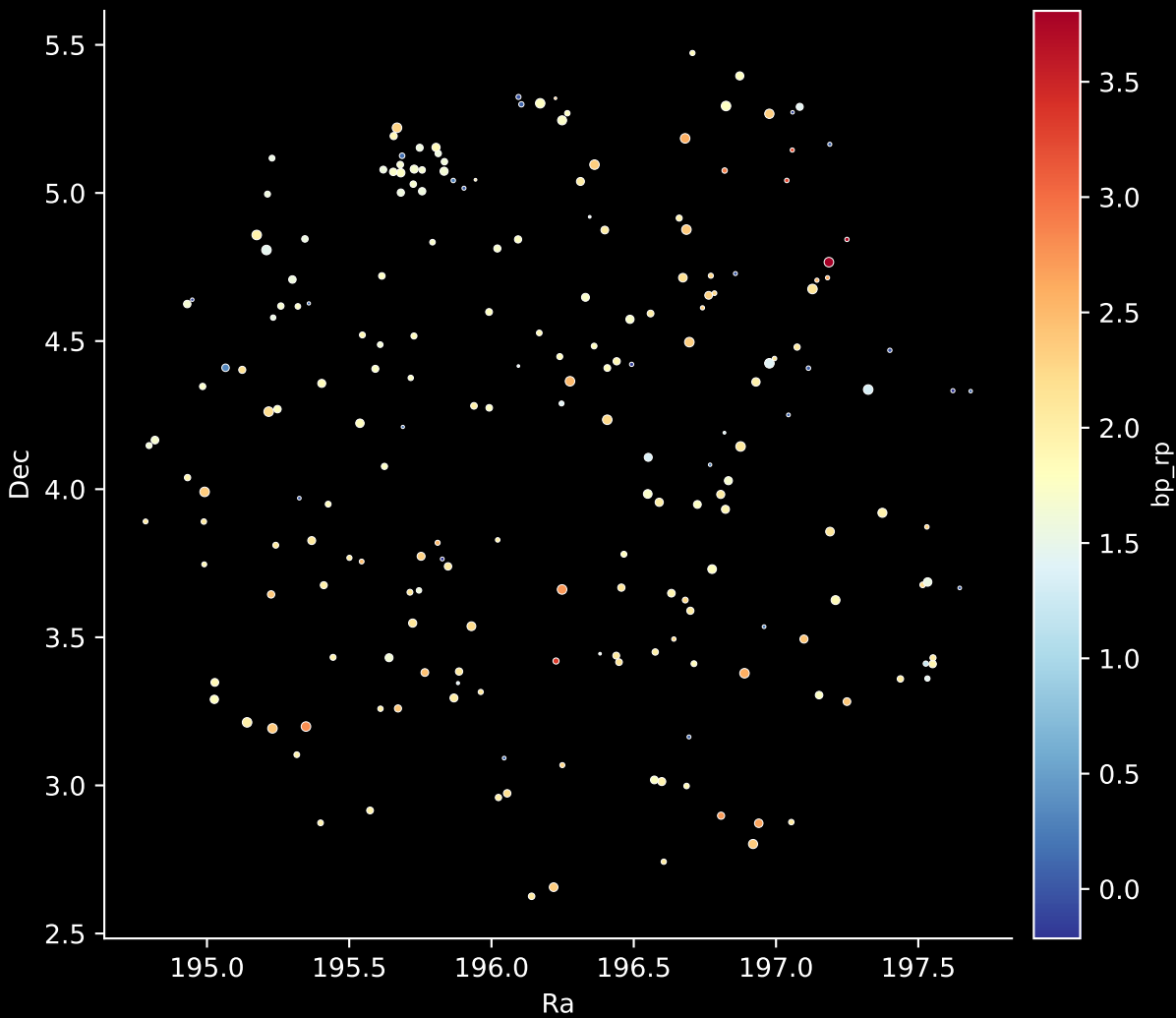
APOGEE DR17 Field: [206-04] Stars: 208
