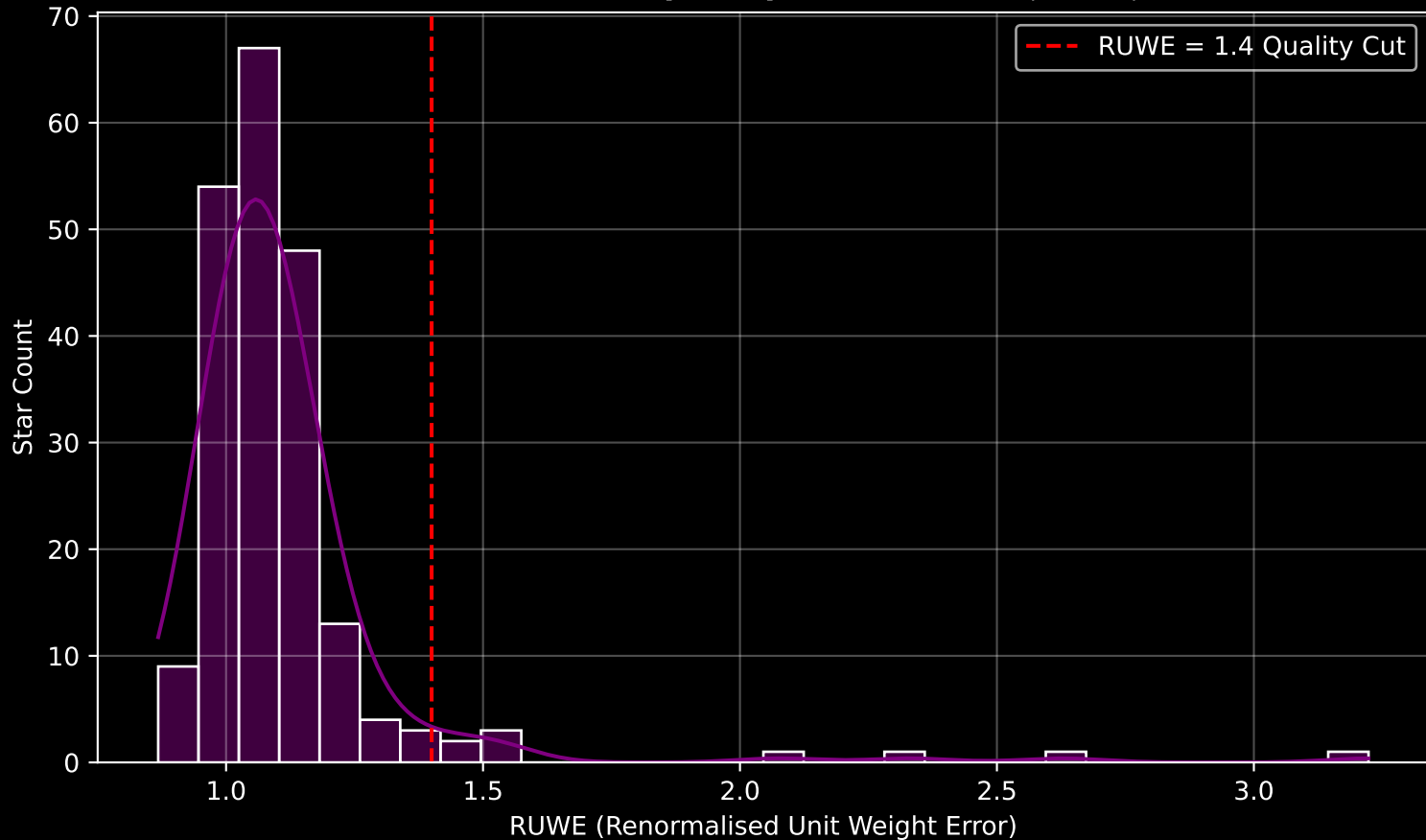
GAPOGEE DR17 Field [206-04] RUWE Distribution (n= 207)
