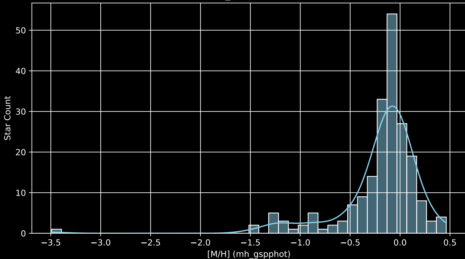
APOGEE DR17 Field: [206-04 [M/H] (mh_gspphot) (n= 203)
