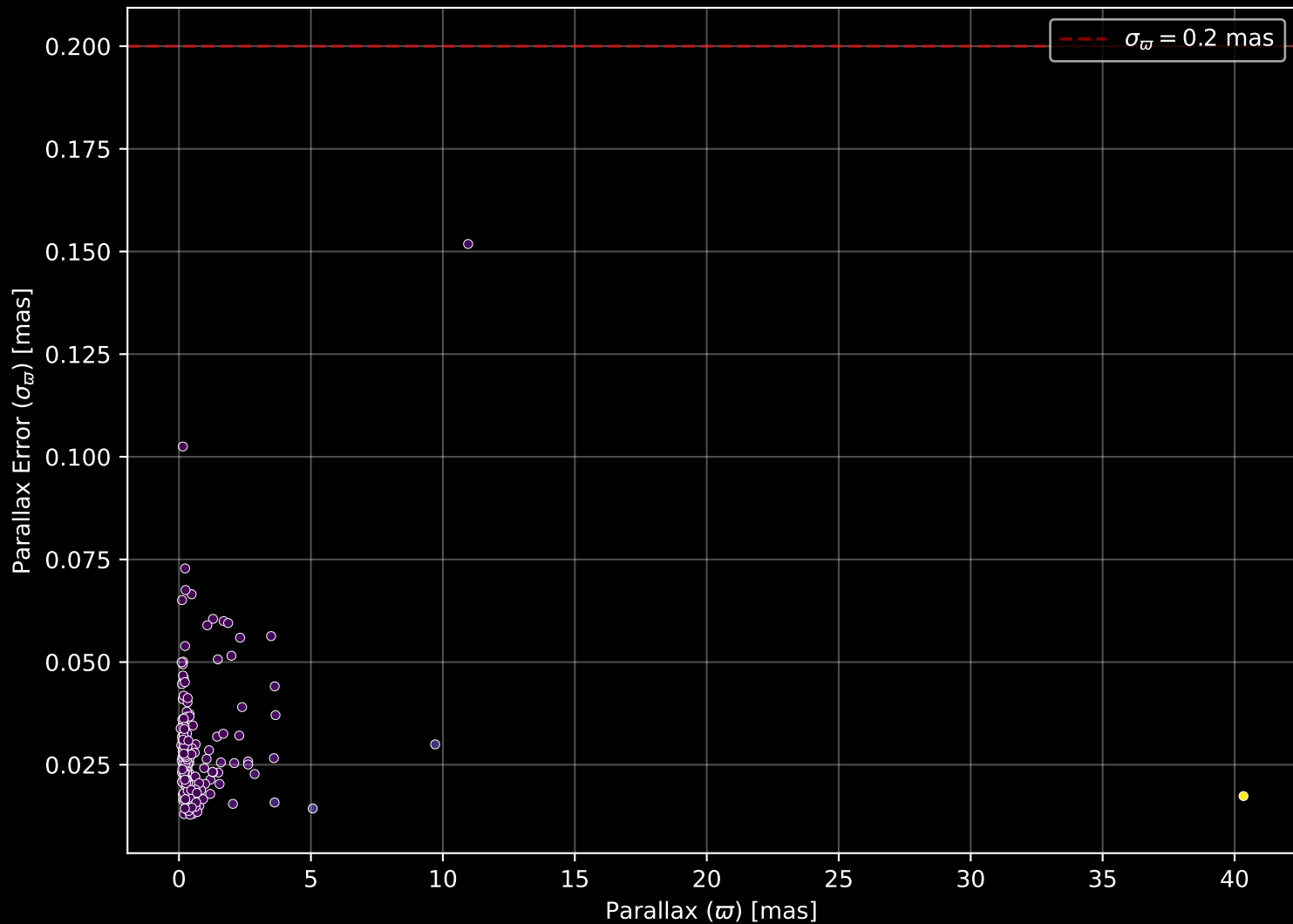
APOGEE DR17 Field: [206-04] Parallax Quality (n= 208)
